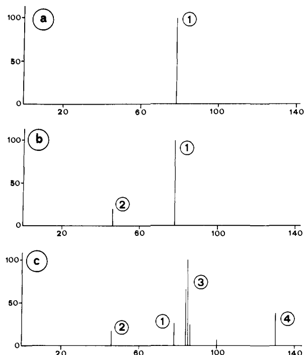
Figure 1. Methane CI of (a) MeNO 3 , low partial pressure (<0.1 mTorr), (b) MeNO 3 , ca. 0.1 mTorr, and (c) MeNO 3 /C 6 D 6 . Major methane peaks (CH 5 + and C 2 H 5 + ) not reported. (1) MeO + (H)NO 2 at m/z 78. (2) NO 2 + at m/z 46. (3) C 6 X 7 + (X = H, D) at m/z 84, 85, 86. (4) C 6 D 6 NO 2 + at m/z 130.
